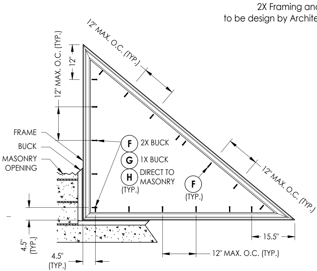
FRAME ANCHORING 76" X 63"
