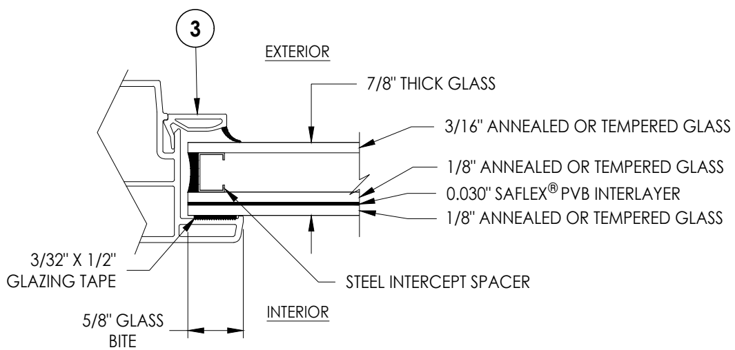
G3 GLAZING DETAIL
